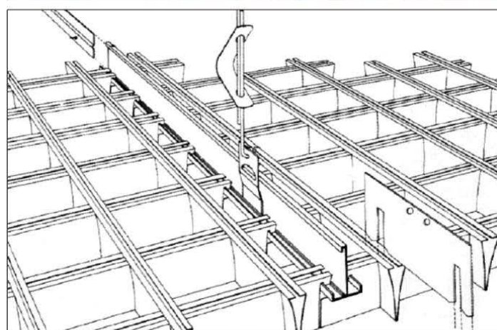
Reflex suspension system
